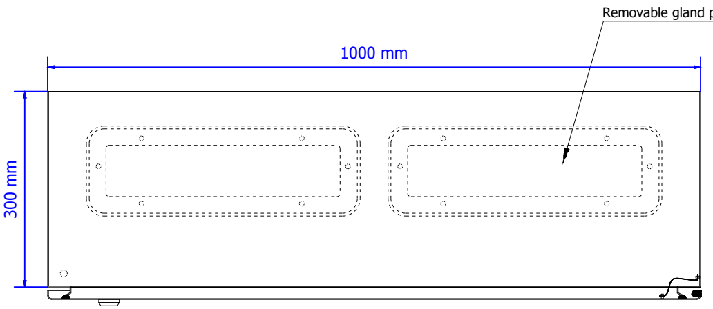
Bottom View
