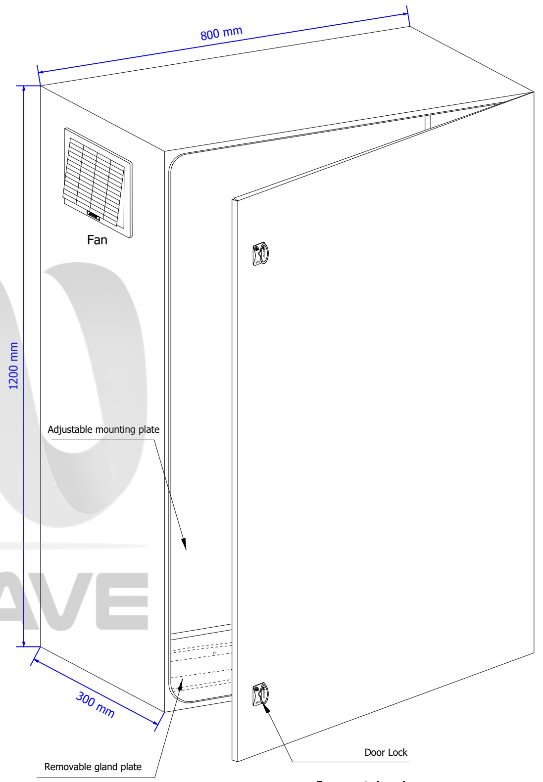
Isometric view
